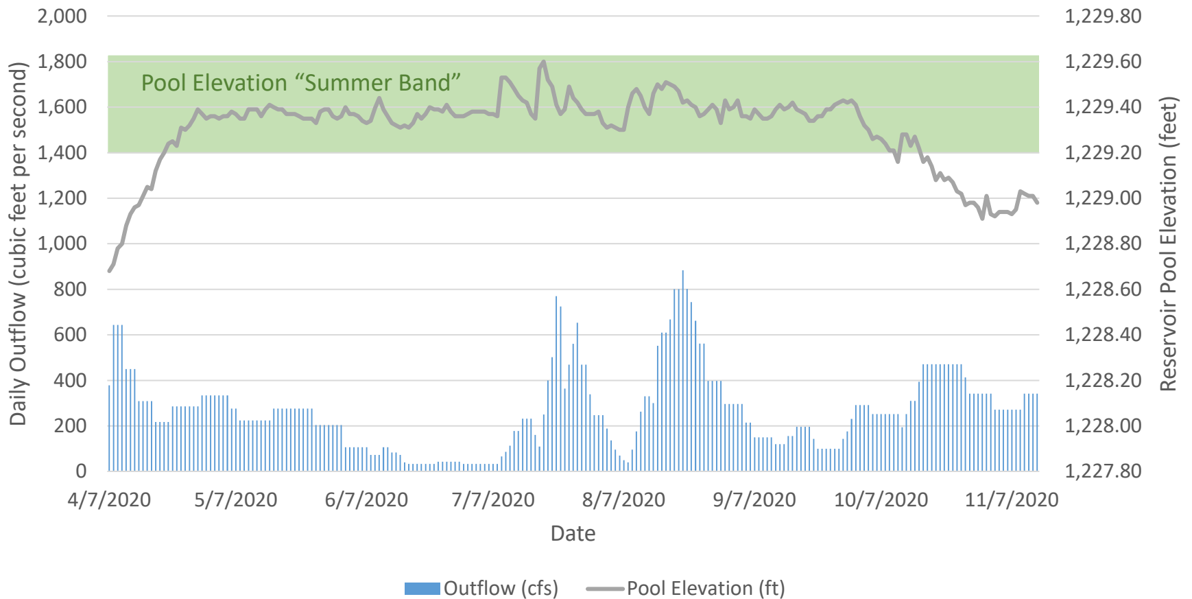
Reservoir Pool Elevation vs. Pine River Dam Outflow
