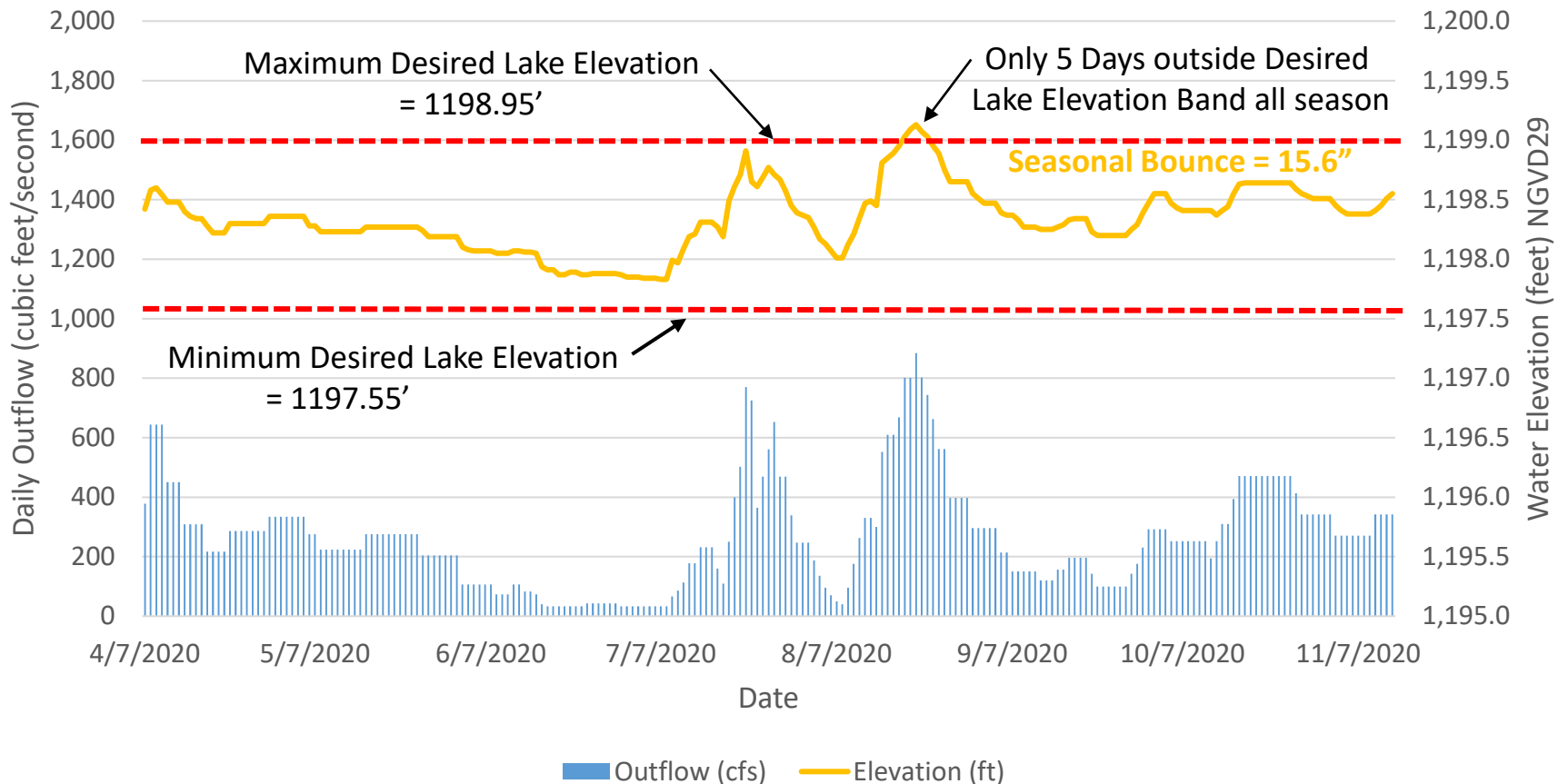
Big Pine Lake Elevation vs. Pine River Dam Outflow
