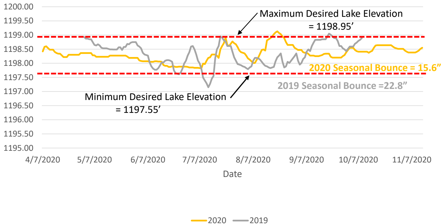
2020 Season vs. 2019 Season Actual Elevations
